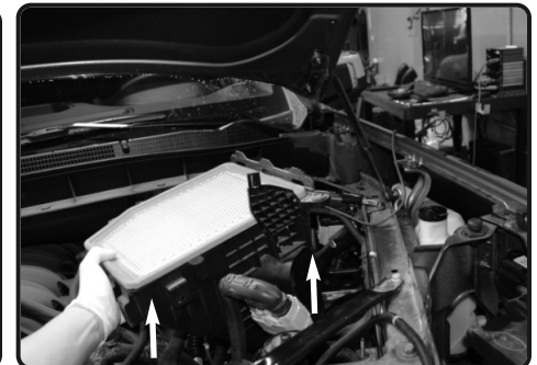
12. Remove the air box, maneuver the box and pull the front inlet to allow the removal. Extra set of hands can come in handy.
