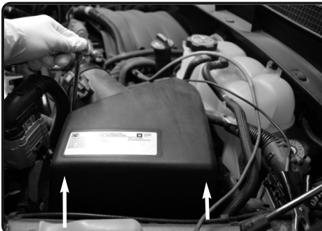
9. Loosen the screws holding in the upper half of the air box. Lift up and remove the upper air box.
