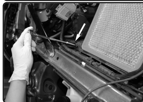
11. Loosen the bolt holding in the lower part of the air box using 10mm socket and ratchet. Save for later install.
