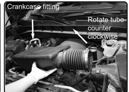
8. Disconnect the crankcase line attached to the intake tube. Rotate the stock intake tube counter clockwise to disengage the keyed mount and then carefully lift up and remove the intake tube out of vehicle.
