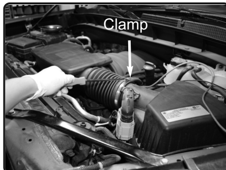
6. Loosen the clamp on the air box using 8mm nut driver.
