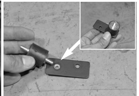
Figure 11 Now install the vibramount to the provided bracket insert. Secure and tighten
