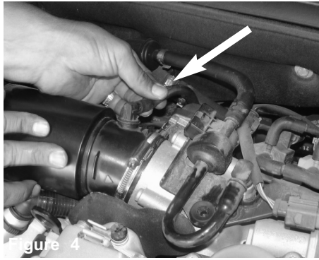
Figure 4 Carefully pull back the vacuum line from the stock intake tube.
