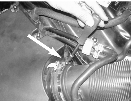
Figure 7 Loosen all the screws holding in the upper part of the air box.
