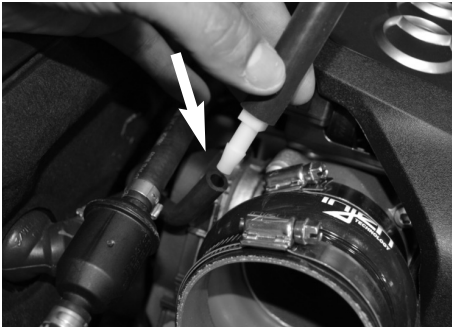
Figure 10 Now attach the coupler extension to the factory vacuum line. Install the 3"-3.25" step hose with clamps to the throttle body. Tighten the clamp on the throttle body only.
