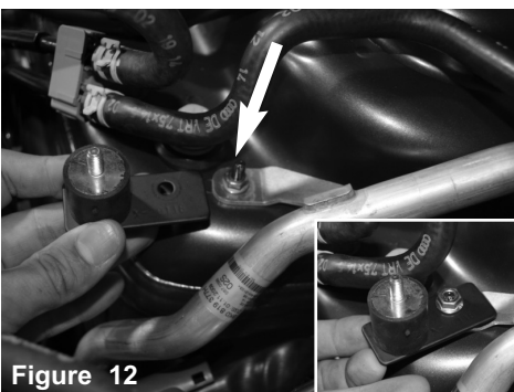
Figure 12 Locate on the strut tower the M6 threaded insert holding the A/C line. Attach the offset side of the bracket to the fitting. Do not tighten.
