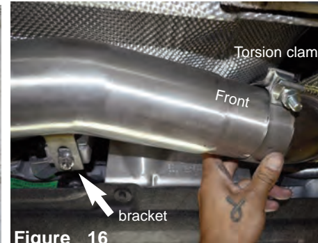
Figure 16 Install the front section to the down pipe and secure using provided torsion clamp. Secure bracket using OEM nut from step Note: Exhaust system has room for adjustment, re-position and tighten for best fit.
