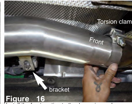
Figure 16 Install the front section to the down pipe and secure using provided torsion clamp. Secure bracket using OEM nut from figure 4 Note: Exhaust system has room for adjustment, re-position and tighten for best fit.
