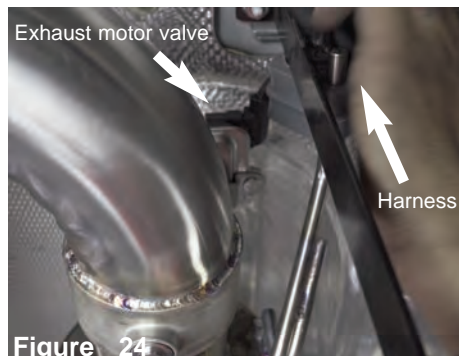
Figure 24 Connect the harness to the exhaust valve motor, run the harness behind the hanger so it will not touch the muffler.
