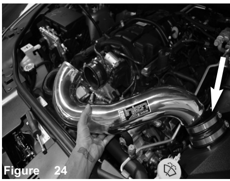
Figure 24 Install the 4.00"-3.50" Step hump hose and two clamps onto the end of the velocity stack and then install the intake tube into the vehicle. Position the tube to the adaptor and the hose on throttle body.
