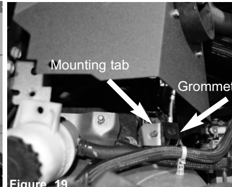
Figure 19 Place the grommet on the heatshield onto the O.E. air box mounting tab on the chassis. Use the power steering reservoir in the photo for reference to locate the mounting tab in the photo.
