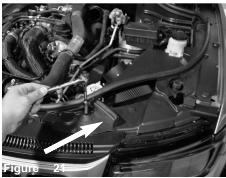
Figure 21 Line up the hole on the bracket of the heatshield to the location where the bolt was removed from figure 6 . Reuse the O.E. 10mm bolt to secure the heatshield bracket to the radiator support.
