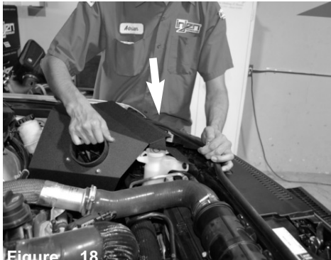
Figure 18 Lift up the plastic radiator support cover and slide the heatshield bracket under it to its mounting position. The mounting position will be the bolt from figure 14 . The heatshield will be secured later.
