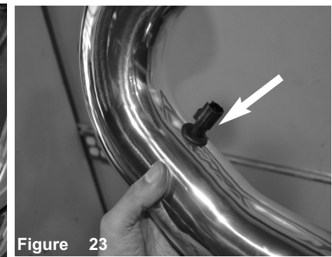
Figure 23 Remove the temperature sensor out of the OEM air-box. Install grommet to the intake tube hole. Now install and secure the Temperature sensor to the grommet.
