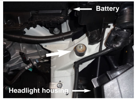
21. Screw the provided vibra mount into the threaded hole located on the chassis in front of the battery and fuse box.
