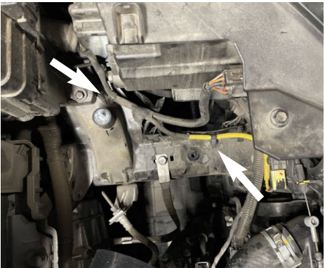
22. Detach both headlight harness to allow clearance for the intake tube.
