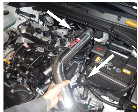
12. Install the intake tube. Insert the tube into the step hose then line up the bracket to the vibra mount.
