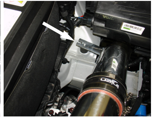
27. Secure both brackets with the provided M6 nut and washer.
