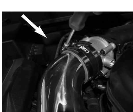
Figure 25 Tighten the clamp on the throttle body using 8mm nut driver.
