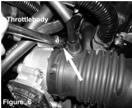
Figure 6 Loosen the clamp on the throttle body using 10mm socket and ratchet. Pull back crankcase line from intake tube.
