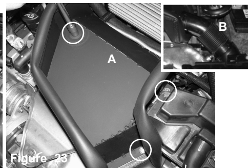
Figure 23 A) Secure the heatshield scoop using provided M6 nuts. Secure and tighten using socket or wrench. B) Now re-install the snorkel scoop from steps 9 & 10 and install to the vehicle and position like image above.
