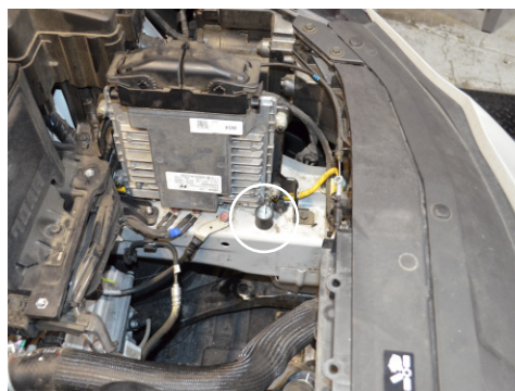
12. Fasten the provided vibra mount onto the threaded hole on the chassis.
