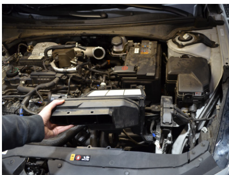
10. Remove the bottom airbox assembly.
