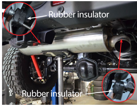
2. Apply lubricant to the rubber insulators, then remove the stock muffler by detaching the hangers from the insulators.
