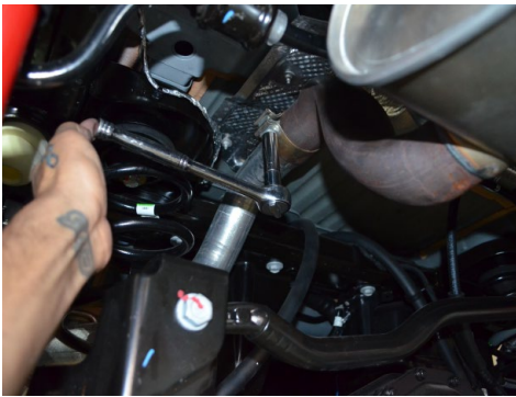
1. Loosen the clamp securing the OEM muffler section.
