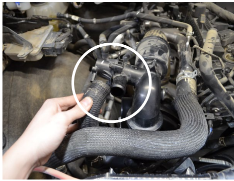
2. Release the tension clamp on the diverter valve outlet hose then detach the diverter valve hose.
