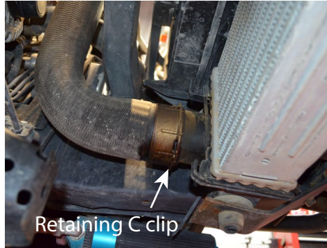
29. Disengage the retaining C clip by prying down on the clip until it snaps into the unlock position. Once released, detach the intercooler hose.
