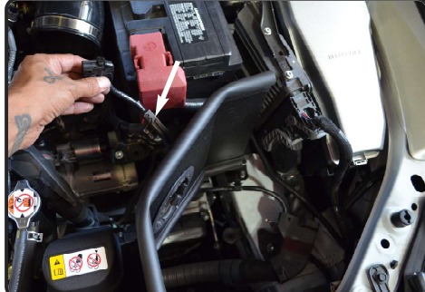
23. Route the MAF harness under the heatshield.
