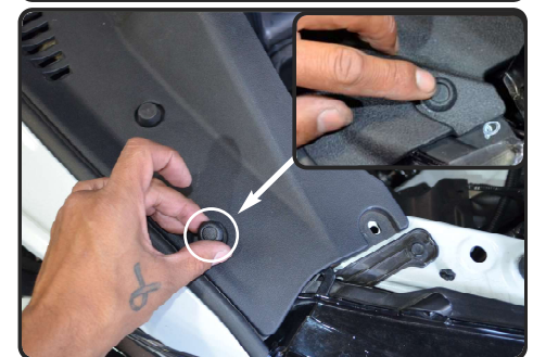
12. push down on the clips on the radiator cover, remove clips and guard for installation of heatshield.
