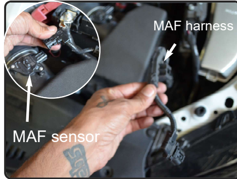
2. Disconnect the MAF sensor harness and pull harness cable from the air box.
