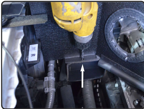
18. Drill hole to 1/4" on the OEM ram scoop.
