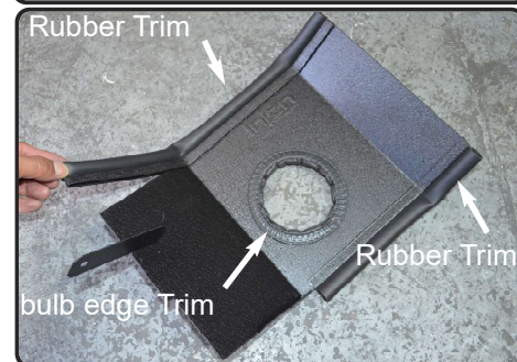
11. Add the Rubber trim to the top and bottom of the heatshield, and the bulb edge trim to hole on heatshield.
