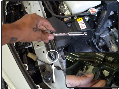
13. Loosen the 1 bolt holding in the OEM Ram scoop. This is where the heatshield will mount to. Remove the 1 grommet from the oem air box mounting brackets.
