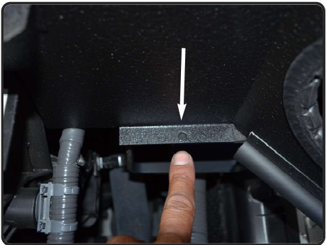
17. Locate the hole on the heatshield smaller tab. now that the OEM Ram scoop is under it, mark hole with marker.
