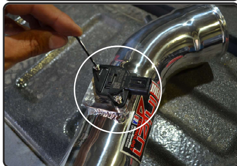
10. Now install the MAF sensor into the new injen intake tube. Secure and tighten using provided M4 button head screws.
