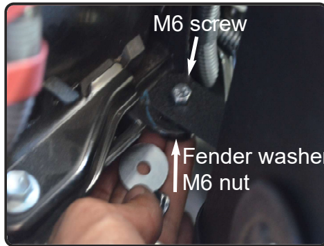
15. Secure the back of heatshield using M6 screw and M6 nut and washer. Make sure Fender washer is secure on the nut side.
