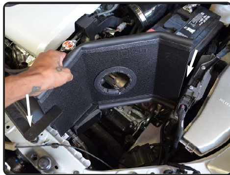
14. Now install the heatshield and position the brackets on heatshield to other mounting points.
