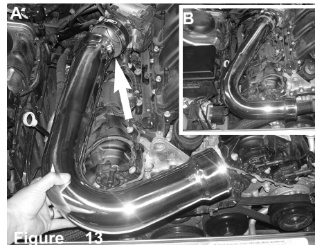
Figure 13 Figure A: Place the primary pipe into the 3/8" hose located on the throttle body. Figure B: Pipe shown in proper position
