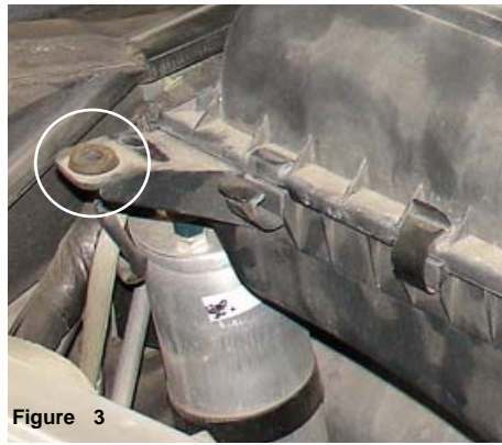
Figure 3 Remove the lock nut located on the mounting bracket that retains the air box cleaner to the fender well.
