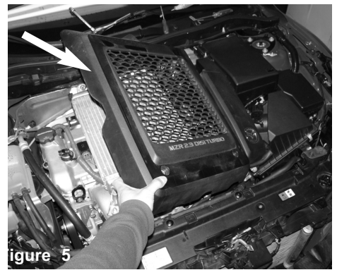
Figure 5 Once you have removed the m6 bolts, continue to remove the intercooler cover.
