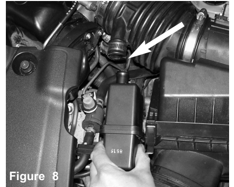
Figure 8 Once you have loosened the small clamp, continue to pull the CCV box from the air intake duct.
