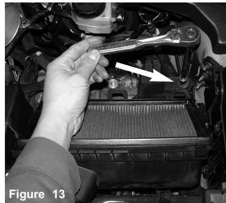
Figure 13 Then m6 bolt holding the air box to the fender well brace is loosened.
