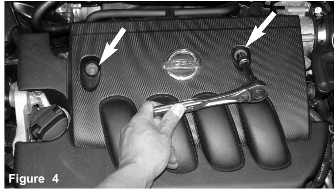
Figure 4 The two m6 bolts are now removed.
