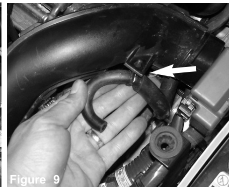
Figure 9 The resonator tube is slightly pulled from the CCV box and the vacuum plastic clip is detached from the tube bracket.
