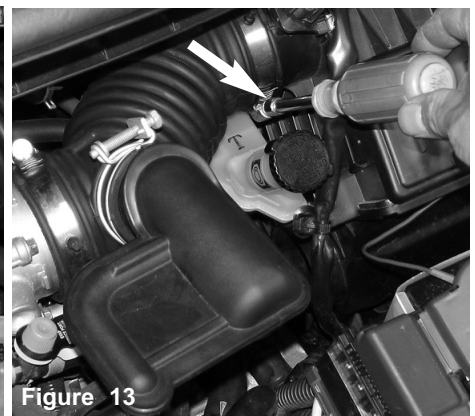
Figure 13 The clamp on the air box side is now loosened as shown above.
