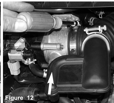
Figure 12 The air duct clamp is loosened at the throttle body, once the clamp has been loosened the air duct, continue to loosen the clamp on the air box side.
