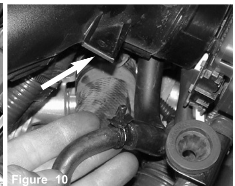
Figure 10 The plastic on vacuum line is removed from the resonator tube.
