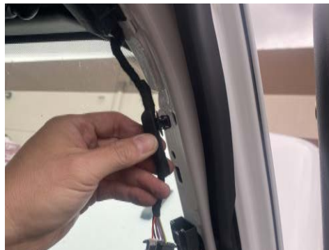
20. Unclip the harness behind the pillar grab handle.
