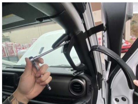
23. Reinstall the pillar grab handle with the upper bracket in place. Reinstall the speaker cover and door seal.
