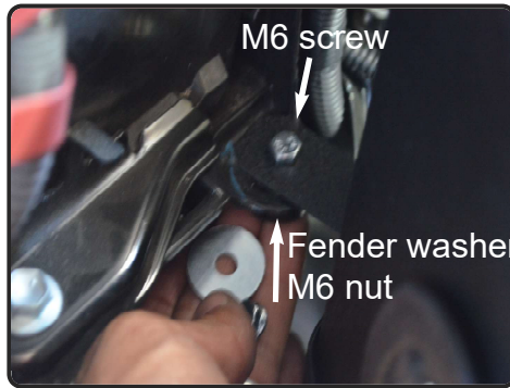
15. Secure the back of heatshield using M6 screw and M6 nut and washer. Make sure Fender washer is secure on the nut side.
