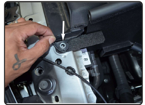
16. Place the tab under the ram scoop and tighten using OEM screw. Secure and tighten.
