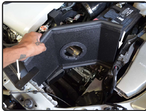
14. Now install the heatshield and position the brackets on heatshield to other mounting points.
