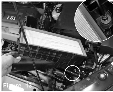
Figure 13 Loosen the bolt on the lower part of the airbox using T30 torx-bit. Carefully remove the lower part of the airbox out of vehicle including the drain line attached to the air box.
