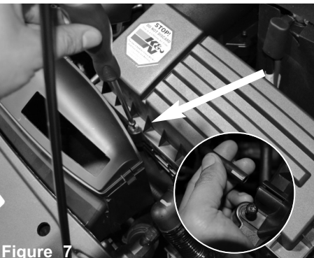
Figure 7 Remove the upper half of the airbox cover. Loosen the screws using phillips screwdriver. Pull back the vacuum line from the stock OEM airbox.
