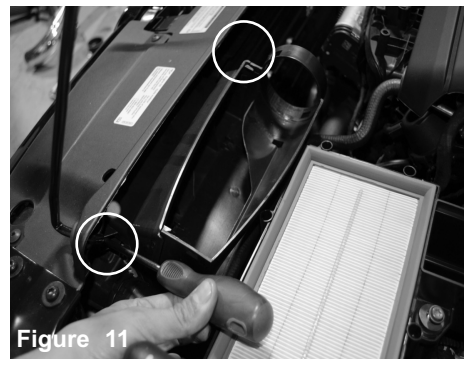
Figure 11 Loosen the 2 screws holding in the ram scoop using T25 torx bit or screwdriver. Save the screws for later install.
