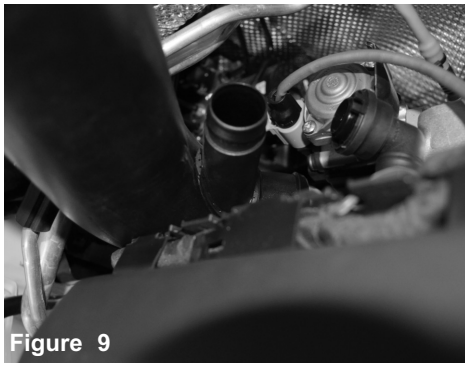
Figure 9 Disconnect the crank-case line from the stock intake tube.
