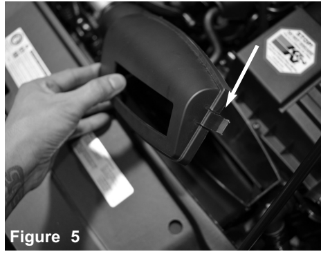
Figure 5 Pull back the scoop/ram cover.
