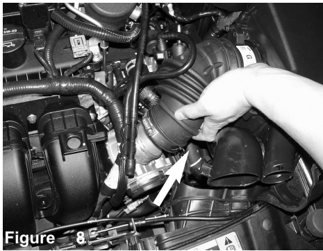
Figure 8 Pull back intake tube from throttle body.
