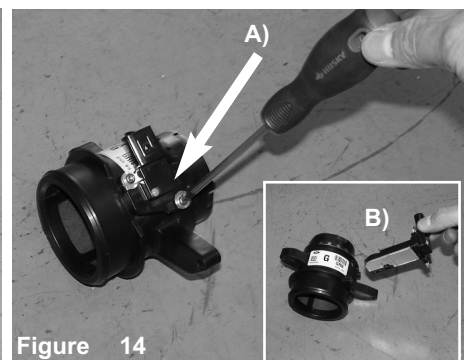
Figure 14 A) With T20 torx screwdriver, loosen the 2 screws holding in the MAF sensor. B) Carefully remove the MAF sensor from the housing.
