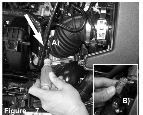
Figure 7 A) With 8mm nut driver, loosen the clamp on throttle body. B) Disconnect the MAF sensor harness.
