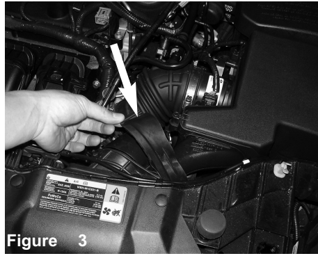
Figure 3 Pull back the rubber clamp holding in the air box to the front of the radiator support.
