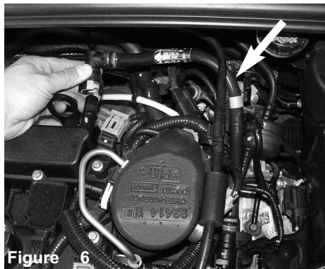
Figure 6 Disconnect the crank case line from engine and remove from vehicle.
