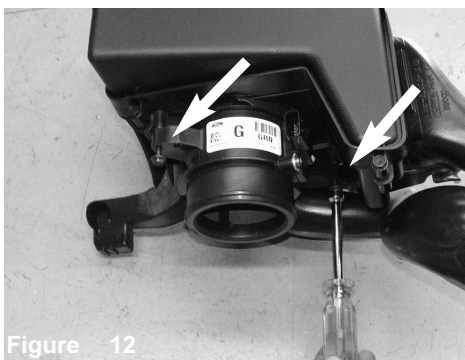
Figure 12 Loosen the 2 screws holding in the MAF sensor housing using 8mm nut driver.
