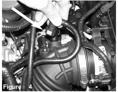
Figure 4 Disconnect the vacuum line from stock intake.
