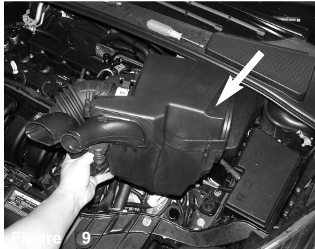
Figure 9 Pull back the ram air scoop from radiator support. Carefully lift and pull out air box.
