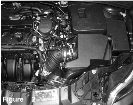
Figure 2 Complete stock air intake cleaner and air intake duct.
