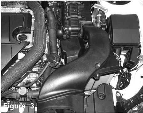
Figure 3 Stock engine compartment. Disconnect the MAF sensor and battery before the installation.
