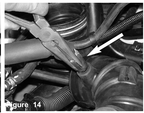
Figure 14 The tension clamp on the crank case line is depressed and removed. Pull back crank case line back from fitting and remove stock intake tube.
