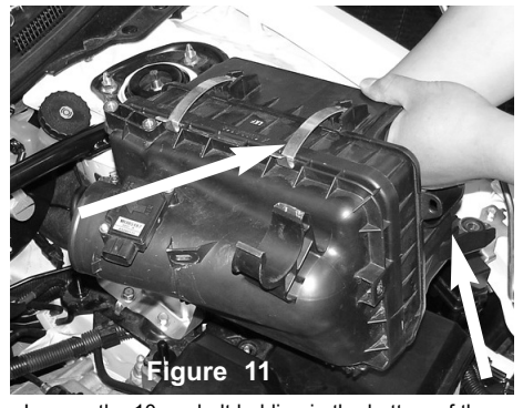
Figure 11 Loosen the 10mm bolt holding in the bottom of the air box. The air box cleaner is ready to be pulled from the engine compartment.
