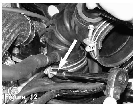
Figure 12 The air duct clamp is loosened connected on the turbo inlet.
