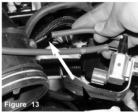
Figure 13 The short vacuum hose on the boost solenoid is disconnected from the air intake duct.
