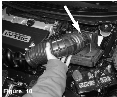
Figure 10 Now pull the upper air box assembly forward and out.
