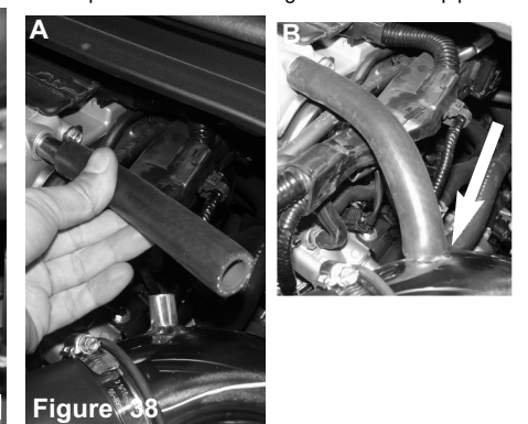
Figure 38 Figure A: Connect the supplied 15mm vacuum line to the crank case vent tube on the valve cover. Figure B: Now connect the other end to the nipple welded on the intake pipe.
