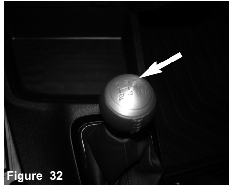
Figure 32 Place the car into 5th gear. The shifter counter weight lever in the engine bay is in its highest position when in 5th gear and you will have to check for pipe clearance later in figure 37
