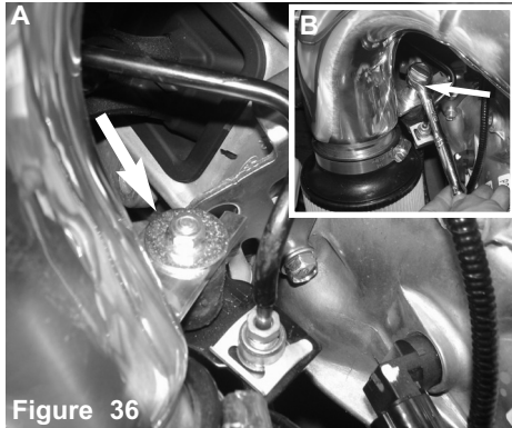
Figure 36 Figure A: Place a fender washer and M6 nut onto the vibramount and intake bracket from figure 34 Figure B: Use a 10mm socket and ratchet to tighten the 10mm nut to the vibramount
