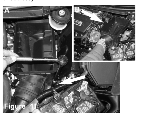
Figure 11 Figure A: Use a 10mm socket and ratchet to remove the bolt on the front right side of the lower air box assembly. Figure B: Lift up on the back side of the lower air box assembly to detach the rear grommets and then pull the lower box assembly out.
