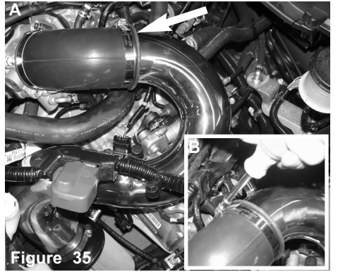
Figure 35 Figure A: Push the intake pipe into the 60 degree elbow. Align the intake for best fitment before securing the clamps. Figure B: Use a 8mm nut driver to tighten the clamp to secure the 60 degree hose to the pipe
