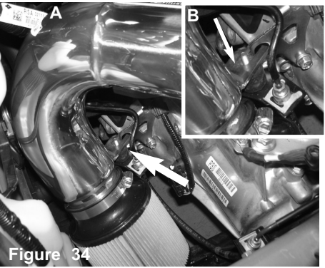
Figure 34 Figure A: Position the intake bracket onto the vibramount from figure 25 and 26 Figure B: Close up of the intake bracket on the vibramount.
