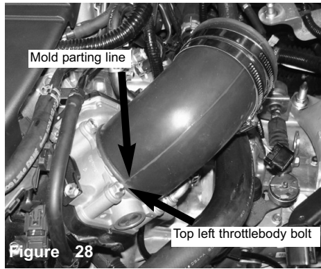
Figure 28 NOTE: Line up the mold parting line on the 60 degree elbow with the top left throttlebody bolt. This will position the 60 degree hose in the correct angle and position prior to installing the intake pipe
