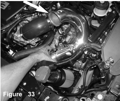
Figure 33 Lower the intake pipe into the engine bay and position the intake pipe to the 60 degree elbow hose.
