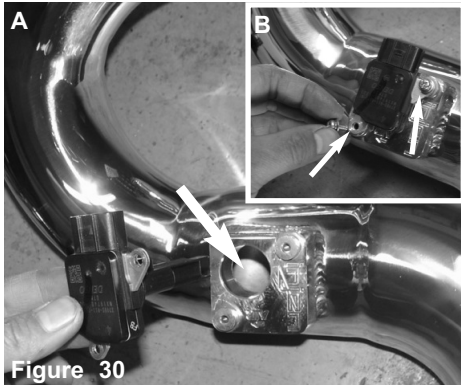
Figure 30 Figure A: Place the stock MAF sensor into the MAF sensor adapter welded on the intake pipe. Figure B: Place the two factory screws onto the MAF sensor
