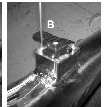
Figure 18 A) Align bracket to vibra mount and secure. B) With provided fender washer and M6 nut secure bracket. Do not tighten.
