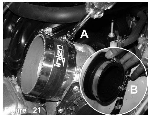
Figure 21 A) Attach 3-1/2" hose with clamps provided to throttle body and tighten on throttle body only. B) Place clamp on elbow hose. Do not tighten.
