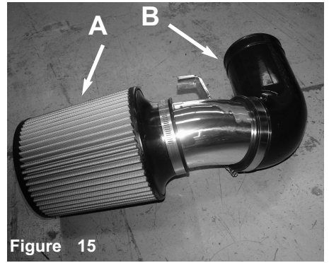
Figure 15 A) Install air filter to lower tube and tighten using 8mm nut driver. B) Install short side of elbow hose to other end of tube with clamp. Do not tighten.
