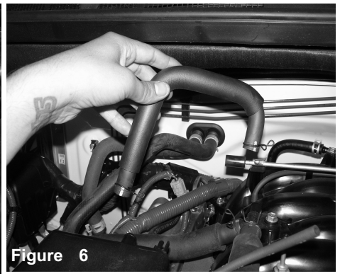
Figure 6 Remove crank case line from vehicle. (will be replaced with provided 15mm hose)
