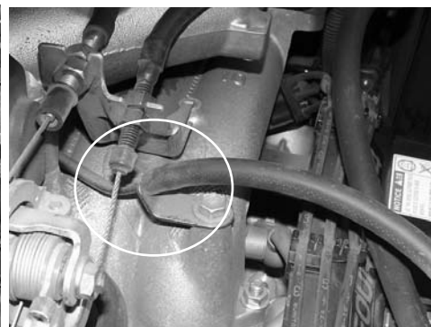
Press the 27" 10mm vacuum hose over the small intake port as shown above. This line will connect to the 3/8" center port nearest to the throttle body.
