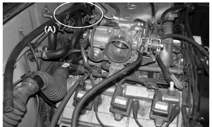
Once you have removed the stock vacuum at the intake port replace it with the Injen 19" 12.5mm vacuum hose (A).
