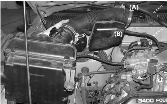
Remove the entire stock air intake box and air intake duct. Disconnect the large 1/2" hose by the firewall (A). The smaller 3/8" hose connected to the intake resonator will also come out intact (B).
