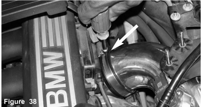
Figure 38 Once the intake is butted with the step hose velocity stack, continue to tighten the step hose clamp.
