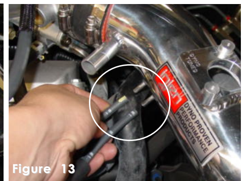
Figure 13 Take the two 4mm vacuum lines and press them into the two small 3/16 vacuum ports on the intake.
