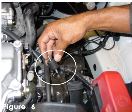
Figure 6 Take the 6mm vibra-mount and screw it into the stock air box bracket. Make sure it is fully screwed into the pre-tapped hole.
