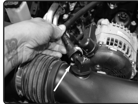
7. Pull back crank case line from air box fitting.
