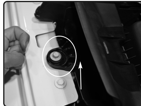
6. Now loosen the 10mm bolt holding in the air box.
