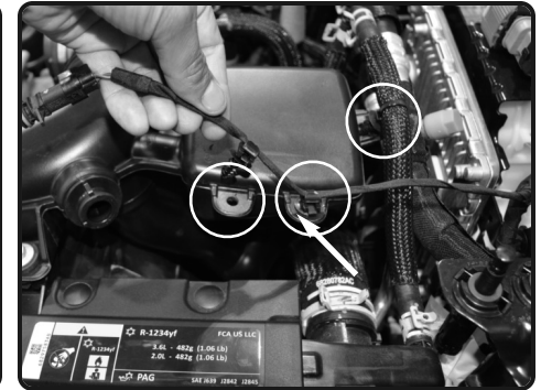
3. Pull back the temperature sensor harness from the intake tube.
