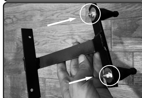
10. Install the provided stand off studs to the bracket and secure using fender washers and nuts. Secure and tighten.
