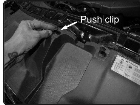
7. Carefully remove the push clips using flat head or panel clip removal tool.
