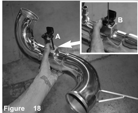
Figure 18 A) Now install the MAF sensor into the intake tube. B) Secure the MAF sensor using provided M4 button head screws.
