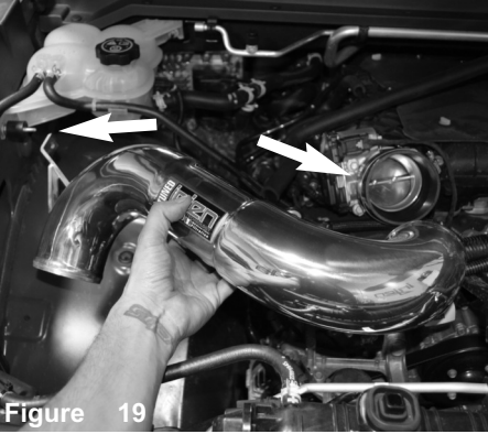
Figure 19 A) Install the intake tube into the vehicle and position the bracket to the vibramount and tube to the step hose.
