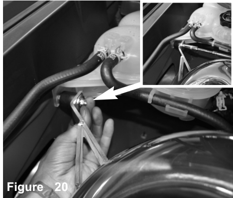
Figure 20 Now secure the bracket using provided nut and fender washer. Secure and tighten using 10mm wrench.
