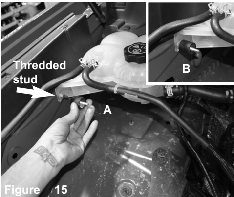
Figure 15 A) Locate the coolant reservoir. Now with provided M6 vibramount, secure to the threaded stud. B) Secure and tighten vibramount.
