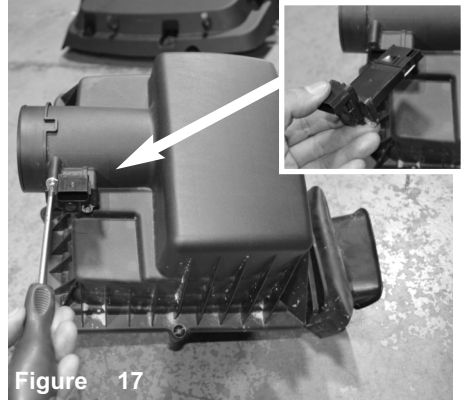
Figure 17 Loosen the 2 screws holding in the MAF sensor using T25 torx bit, and remove sensor from vehicle.
