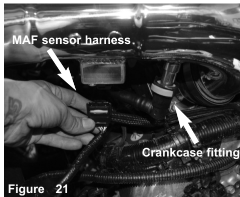
Figure 21 Connect the crankcase line to the fitting on intake tube. Re-connect the MAF sensor harness. Make sure you hear a click for both to be secured properly.
