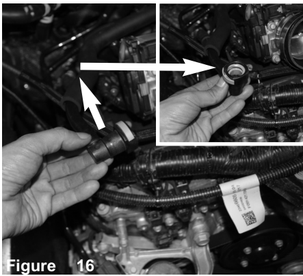
Figure 16 Locate the plastic crankcase fitting, rotate 90 degree so fitting is sitting up.
