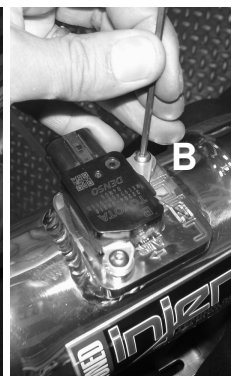
Figure 26 A) Install the MAF sensor to the intake tube. B) Now secure using 2.5mm button head screws provided.
