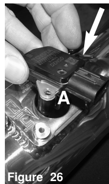
Figure 26 A) Install the MAF sensor to the intake tube. B) Now secure using 2.5mm button head screws provided.
