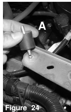
Figure 24 A) Install the vibra mount to the end of the stock air box bracket. B) Secure and tighten.
