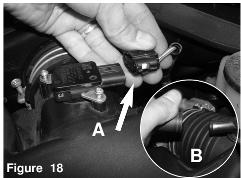
Figure 18 A) Disconnect the MAF sensor harness. B) Pull back the crank case line.
