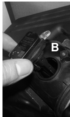
Figure 25 A) Loosen the 2 screws holding in the MAF sensor. B) Remove MAF sensor.
