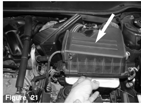
Figure 21 Lift up and remove the upper half of the air box assembly from the vehicle.
