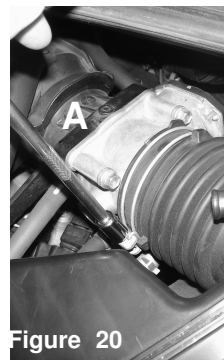
Figure 20 A) Loosen the clamp on the throttle body using 10mm socket or ratchet. B) Pull back any lines from the stock intake system that are attached.
