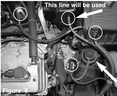
Figure 6 Now for the next few steps we are going to focus on the VAD which you will not use in the new Injen Short Ram. Line shown above will be the only line used in the injen intake system.
