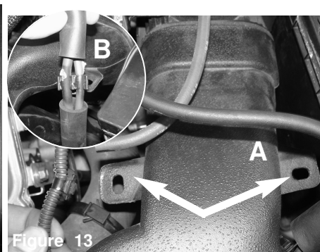
Figure 13 A) Pull harness lines away from the stock ram unit. B) Carefully pull lines away from the ram unit.
