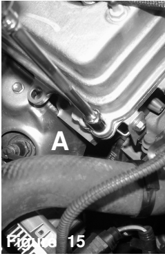
Figure 15 A) Loosen the bolt on the valve cover closes to the VAD module using 10mm socket and ratchet. B) Remove bolt and save for later install.
