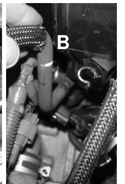
Figure 20 A) Loosen the clamp on the throttle body using 10mm socket or ratchet. B) Pull back any lines from the stock intake system that are attached.
