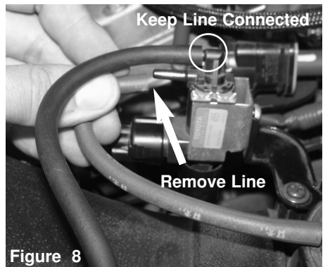
Figure 8 Now image above shows the side of the VAD module. Disconnect the bottom or grey line from the actuator. Leave the top line or black line connected.
