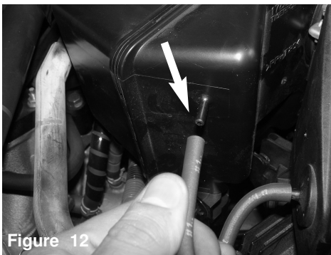
Figure 12 Now remove the remaining last vacuum line from the stock intake system. Note: This line will be used on the injen intake system.
