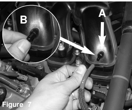
Figure 7 A) Remove the vacuum line from the engine side on the intake manifold fitting. B) Now cap-off fitting using provided medium vinyl cap. Leave the line attached to stock air box so you will not lose it.
