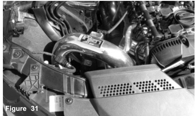
Install the air filter to the tube and tighten using 8mm nut driver.
