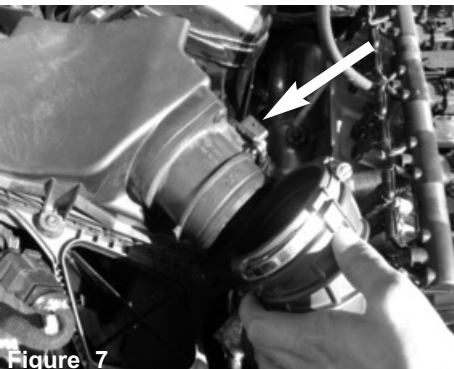
Figure 7 Pull back the factory intake tube.
