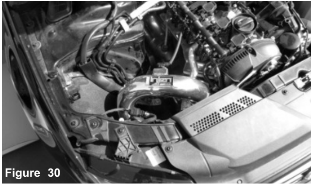
Install the air filter to the tube and tighten using 8mm nut driver.
