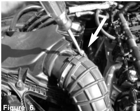
Figure 6 With flat head screw driver, loosen clamp.
