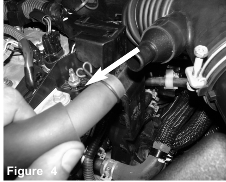
Figure 4 Pull back the crank case line from stock intake tube.
