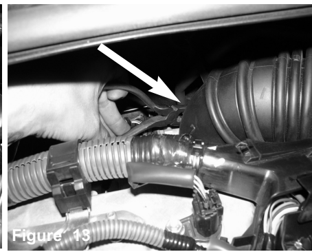
Figure 13 With pliers, pinch the clamp on throttle body.
