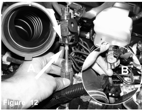
Figure 12 A) With phillips screwdriver, loosen the screw holding in VSV valve on bracket. B) Carefully pull away from tube.
