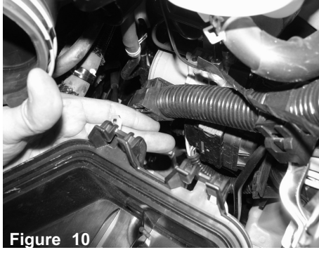
Figure 10 Pull back the ECU harness that is attached to the back of the bottom half of air box.
