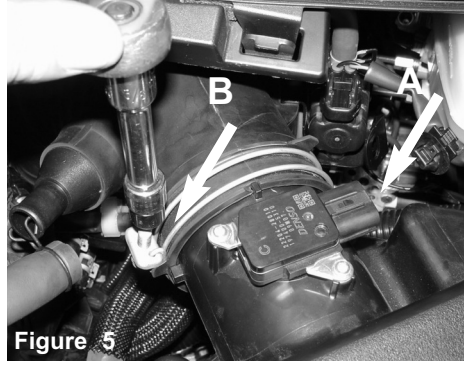
Figure 5 A) Disconnect the MAF sensor harness and harness clips attached to the intake tube. B) Loosen the clamp on air box using 10mm socket or wrench.
