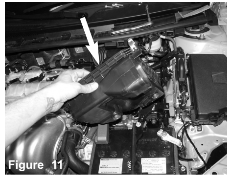
Figure 11 Remove the bottom half of air box out of vehicle.
