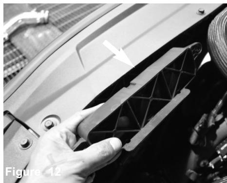
Figure 12 Loosen the 2 bolts holding in the front scoop vent and remove. Save 1 screw for later install.
