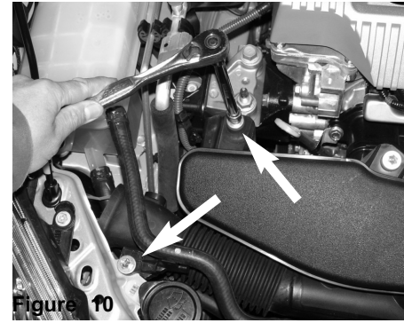
Figure 10 Remove the last two 10 mm bolts attached to the lower airbox cleaner.
