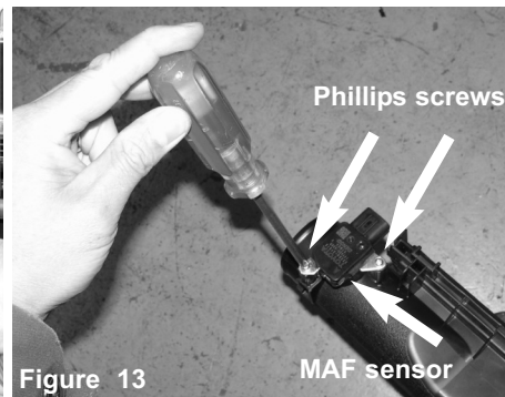
Figure 13 Use a phillips screw driver and remove the two screws attaching the MAF sensor to the upper airbox cover.
