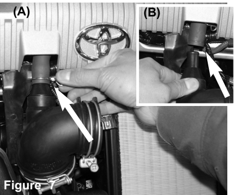
Figure 7 Figure A: Press on the pressure clamp on the air duct breather port. Figure B: Disconnect the breather line from breather duct on the air duct tube.
