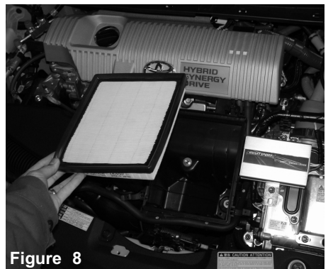
Figure 8 Remove the air filter panel to access the two 10mm bolts attaching the lower airbox cleaner to the engine.
