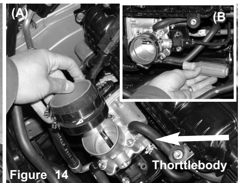
Figure 14 Figure A: Place the 2.5" straight hose and two .040 clamps onto the throttlebody. Figure B: Use an 8mm nut driver to tighten the throttlebody clamp for now.
