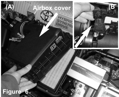
Figure 6 Figure A: Lift up on the airbox cover. Figure B: Disconnect the MAF sensor harness from the MAF sensor on the airbox cleaner.
