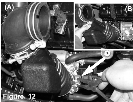
Figure 12 Figure A: Use a set of middle nose pliers and loosen the pressure clamp on the throttlebody air duct. Figure B: Now remove the throttlebody air duct.
