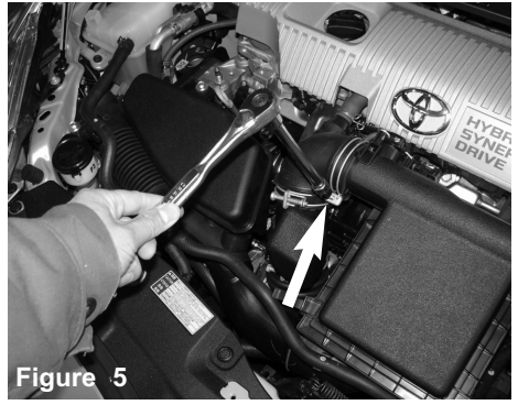
Figure 5 Loosen clamp from throttlebody air duct to air box cleaner using a 10mm socket and 3/8 ratchet
