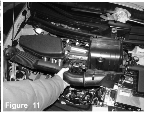
Figure 11 you may now remove the entire lower portion of the airbox cleaner.
