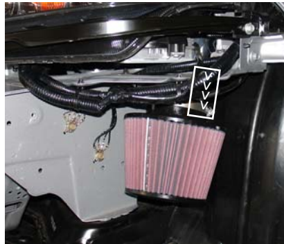
Press the Injen filter over the end of the secondary intake and tighten the clamp on the filter neck.
