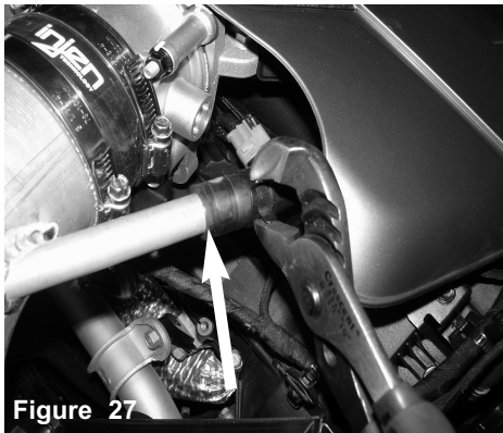
Figure 27 Attach the crank case line to the fitting on the intake tube using pliers and secure.
