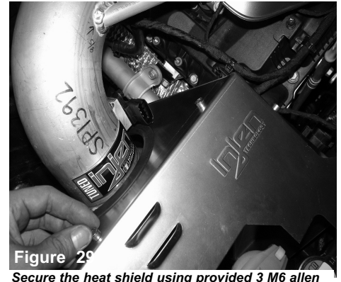
Figure 29 Secure the heat shield using provided 3 M6 allen screws, and tighten.
