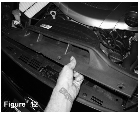
Figure 12 Remove the scoop, this will be used again in the new injen intake system.
