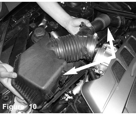
Figure 10 Un-clip the upper part of the air box and remove from the vehicle, including the resonator tube.
