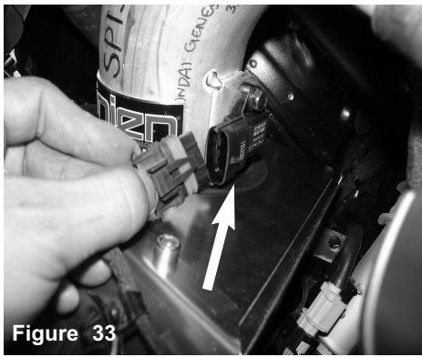
Figure 33 Connect the Temperature sensor harness.
