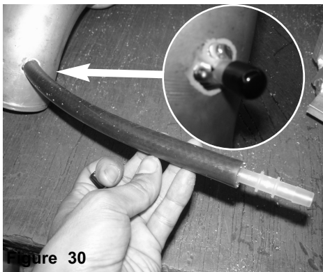
Figure 30 Manual transmission cap off 3/8" fitting using provided 3/8" vinyl cap. Auto transmission connect the 3/8" coupler to factory hose, attach the provided 10mm hose to the 3/8" fitting.
