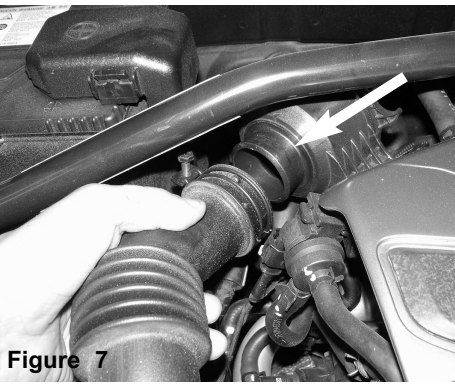
Figure 7 Pull back the sound tube from the resonator. Disconnect the brake booster line if equipped.
