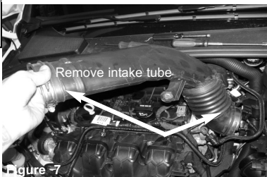
Figure 7 Carefully lift up and remove the stock intake tube from the vehicle.
