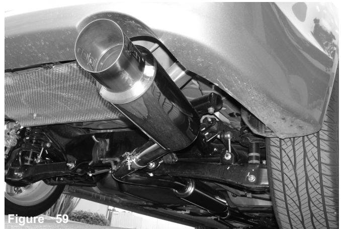
Figure 59 Passenger under shot of the full cat-back system.
