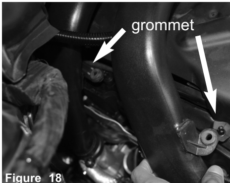
Figure 18 Lift up and pull charge pipe out of the grommet. Lift up and remove from vehicle. Repeat on the other charge pipe.
