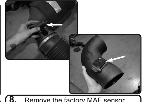
8. Remove the factory MAF sensor from the factory air box assembly and then install it into the Injen intake tube. Use two M4 supplied bolts to secure it to the tube.
