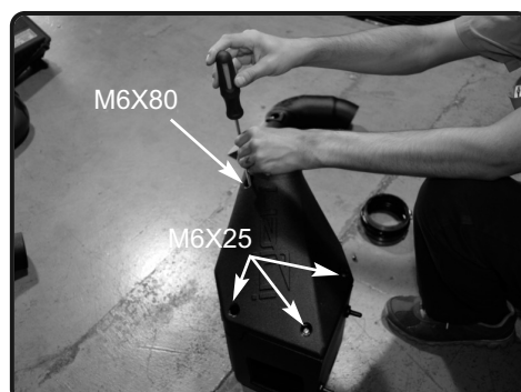
6. Place the three M6X25mm bolts and one M6X80mm into the plenum illustrated by the photo. Your Injen air box assembly is now complete.
