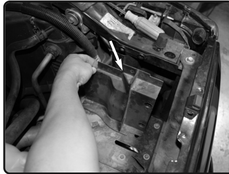
3. Remove the trim panel behind the passenger side headlight. Removing this panel will allow additional air into the intake system.
