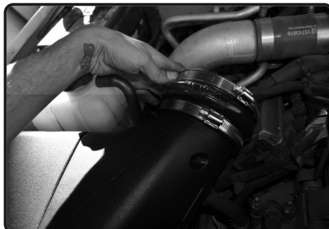
9. Place the 4.50" hump hose and two #80 clamps onto the Injen intake plenum. Secure the clamp on the plenum side for now.
