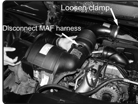
2. Disconnect the MAF sensor harness. Then loosen the clamp on the turbo inlet. Pull the entire air box assembly and air duct out of the engine bay.
