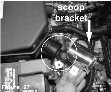
Figure 27 Tighten the scoop bracket using 10mm socket and ratchet.
