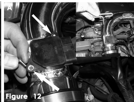
Figure A: Place 2 M4x10 button head screws onto the MAF sensor Figure B: Tighten the M4 bolt with a 2.5mm allen driver
