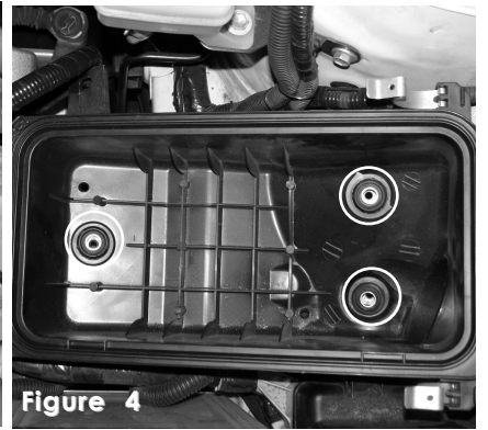
Figure 4 Unscrew the three m6 bolts from the lower air box cleaner. Note: This lower air box cleaner is used for illustration purposes only.
