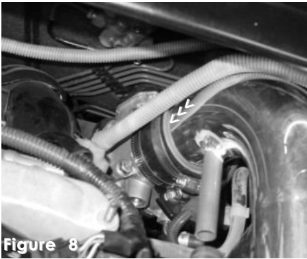
Figure 8 Place the intake in the engine compartment and insert the top end in the throttle body hose.
