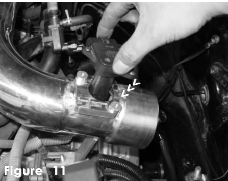
Figure 11 Insert the MAF sensor into the machined intake adapter.
