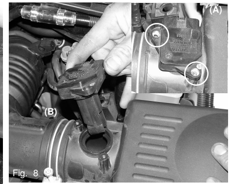
Fig. 8 Unscrew the two screws that secures the mass air flow sensor to the sensor housing (A). Pull the mass air flow sensor up and out of the sensor housing as shown above (B), to be used later in the instruction.
