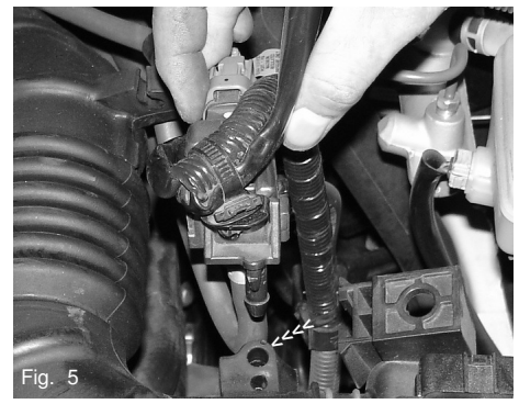
Fig. 5 Pull the entire vacuum switching valve from the rubber saddle on the air intake duct used to secure the vacuum switching valve.
