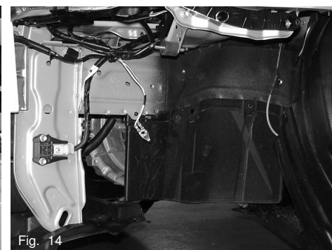
Fig. 14 Remove the entire front bumper by removing all bolts and plastic clips holding the bumper in place.
