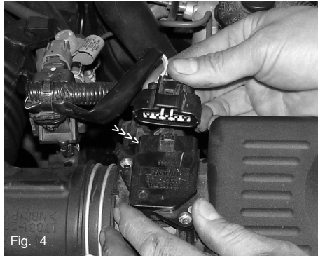
Fig. 4 Disconnect the mass air flow sensor electrical harness from the sensor.
