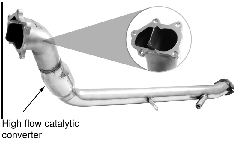
SES1204DP - Full 76mm down pipe and stainless steel cast turbo bellow with divided wastegate discharge.
