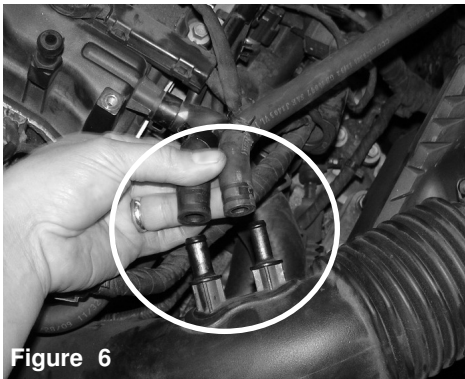
Figure 6 Both breather lines removed from air duct
