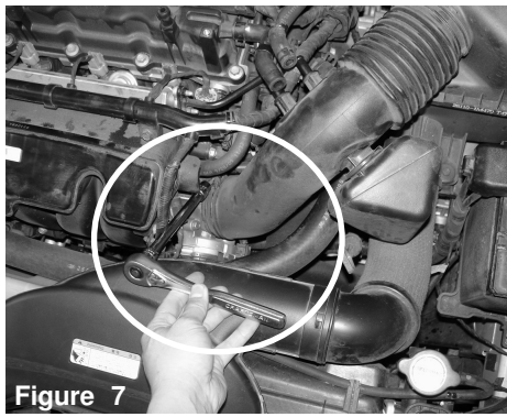
Figure 7 Use a 10mm socket and ratchet to loosen the clamp on the air duct connected to the throttle body
