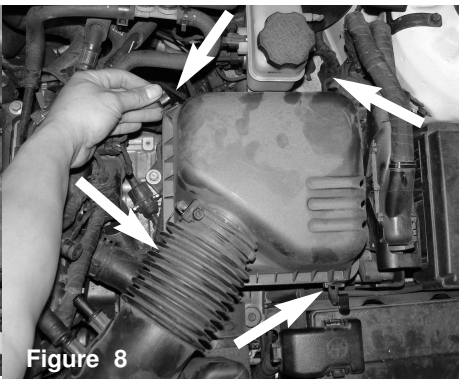
Figure 8 There are four retaining clips that you will have to unlatch to remove the upper portion of the factory air box cleaner
