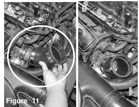
Figure 11 Figure A: Place the 2.75"X3.00" 45 degree elbow with two 48 clamps onto the throttle body. Make sure the 2.75" side goes onto the throttle body. Figure B: Hose shown on throttle body
