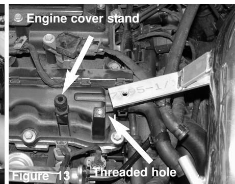
Figure 13 Line up the intake bracket next to the threaded insert on the valve cover next to the engine cover stand
